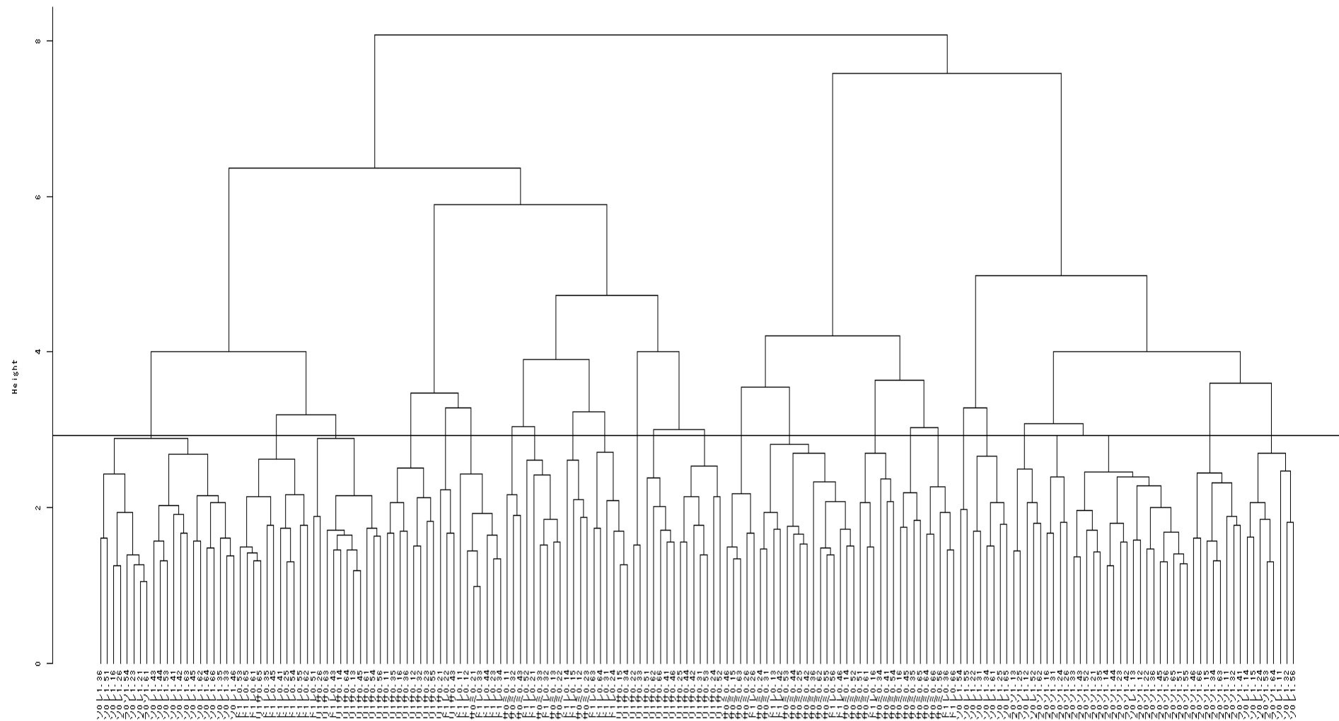
Cluster Dendrogram
