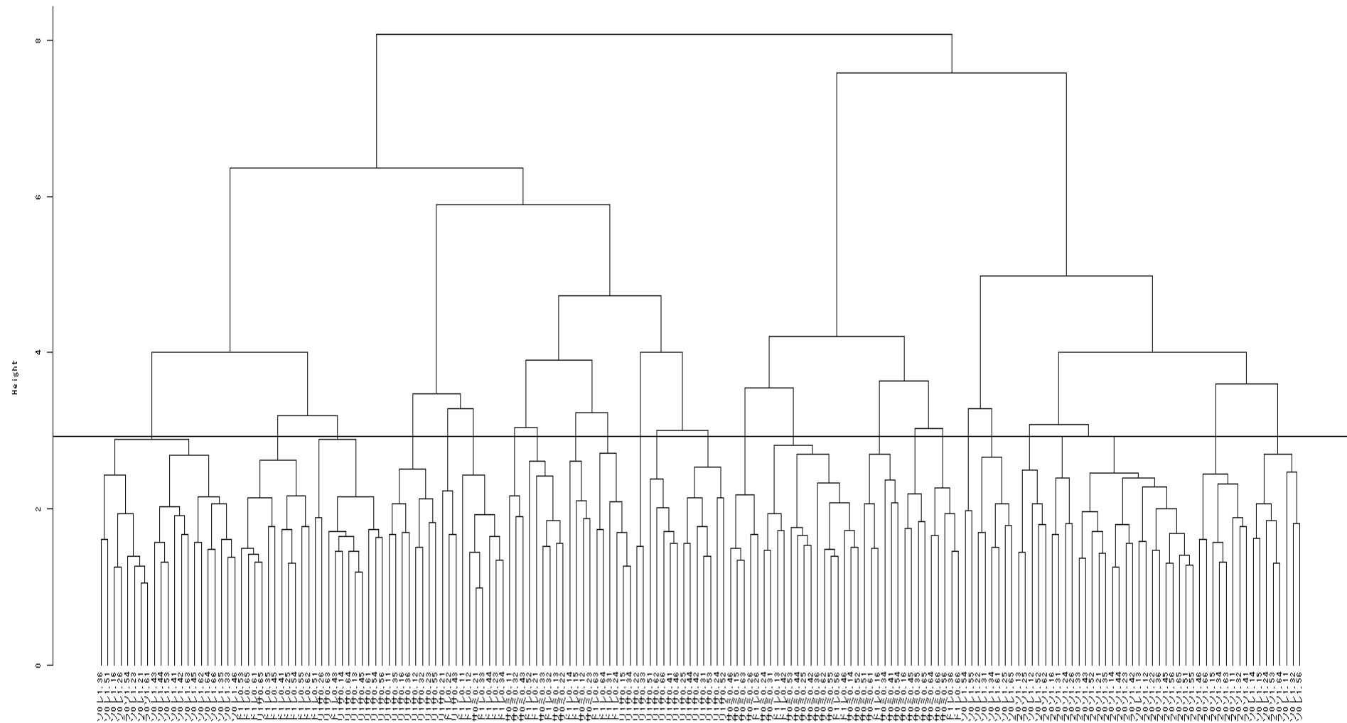
Cluster Dendrogram
